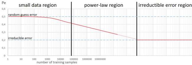
Fig. 2: Schematic generic evolution of the test error depending on the dataset size.
